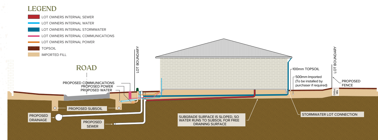
Example diagram of drainage works
